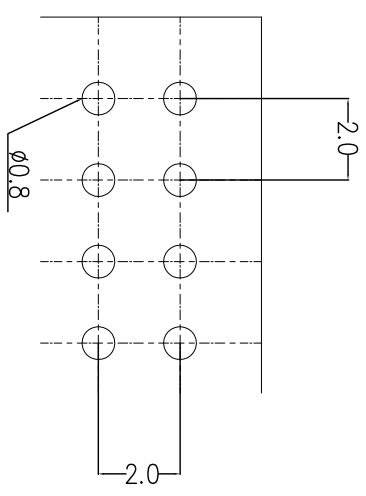
PCB Hole Layout
