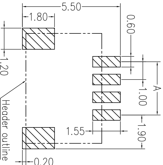
PCB Layout
