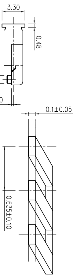
DETAIL "A" 10:1
